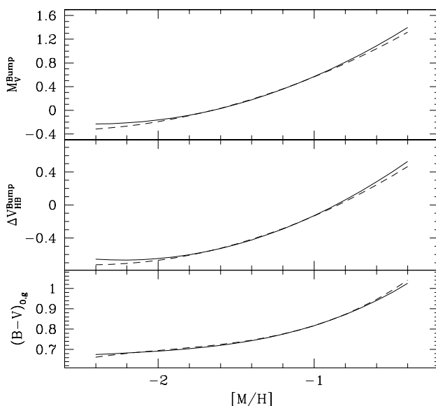
FIG. 23.— (B-V)_{0,g} , \Delta V_{\text{HB}}^{\text{bump}} , and M_V^{\text{bump}} as functions of the global metallicity, computed by adopting the \alpha -enhancement relation plotted in Fig. 1a (solid lines) and adopting the \alpha -enhancement scenario proposed by Carney (1996) plotted in Fig. 1b (dashed lines). As can be seen, the two different assumptions have a very small effect on the derived relations.
