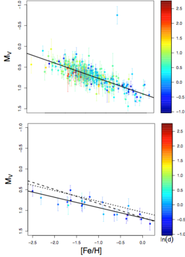
FIGURE 3.34: Top panel : M_V - [\text{Fe}/\text{H}] relation defined by the 381 RRLs in our sample. The absolute magnitudes M_V were inferred from the BA model. The solid line represents the linear fit. Its slope and zero-point are summarised in Table A.4 (first row). The colour scale encodes the (natural) logarithm of the inferred distance measured in units of kpc. Bottom panel : Same as in the top panel but for a sample of 23 RRLs with metallicity from high resolution spectroscopy. Figures from Muraveva et al. (2018b).
