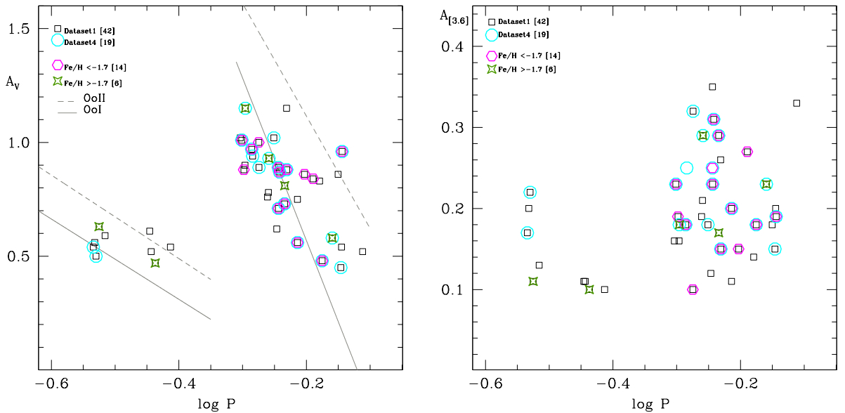
FIGURE 4.16: Left panel: V-band period-amplitude diagram for the 42 RRLs of Sculptor, periods and amplitudes are from K95 and C05. The grey lines mark the loci of the OoI (solid) and OoII (dashed) Galactic GCs from Clement & Rowe (2000) where, typically, OoI systems are more metal-rich ( [\text{Fe}/\text{H}] \sim -1.5 dex) than the OoII systems ( [\text{Fe}/\text{H}] \sim -2 dex). Black empty squares are the D1 sample while cyan circles are the D4 sample. Magenta hexagons and green four-pointed stars denote metal-poor and metal-rich samples, according to C05 metallicities. Right panel: MIR period-amplitude diagram, adopting the amplitudes at 3.6 \mu\text{m} derived in this study. Colours and symbols as on the left panel. Figure from Garofalo et al. (2018).
