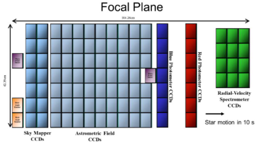
FIGURE 3.3: Gaia CCD array layout. Different colours indicate different functions of CCDs and sensors: purple and orange for the wave-front sensor (WFS) and BAM; CCDs of the SM and the AF, devoted to astrometric measurements are in cyan and light-cyan while the CCDs for the BP and RP are in blue and red respectively. Green for CCDs dedicated to the RVS. Image from http://sci.esa.int/gaia . Credit: ESA - A. Short.
