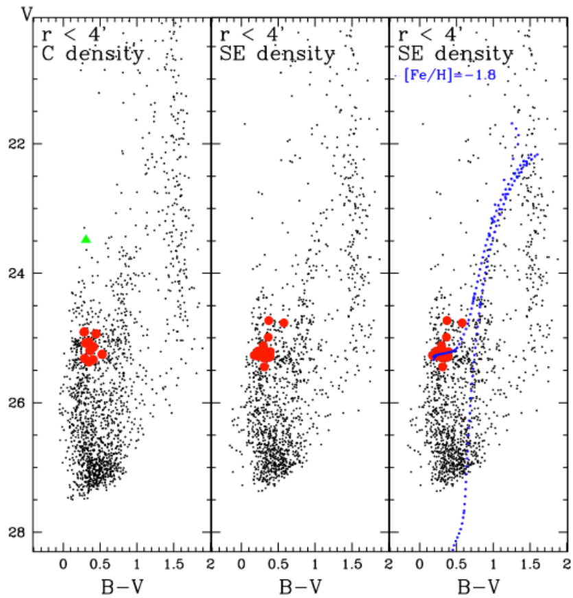
FIGURE 2.35: CMDs of the sources in the C and SE regions. Only objects satisfying the DAOPHOT quality image parameter conditions: -0.35 \leq \text{Sharpness} \leq 0.35 and \chi < 1 are displayed. Red filled circles are the RRLs, a green filled triangle is the AC. Left panel : CMD of the sources in the C region. Middle panel : CMD of the sources in the SE region. Right panel : Same as in the middle panel but with superimposed a stellar isochrone of 13 Gyr with [\text{Fe}/\text{H}] = -1.8 dex (blue dotted line; see text for details).
