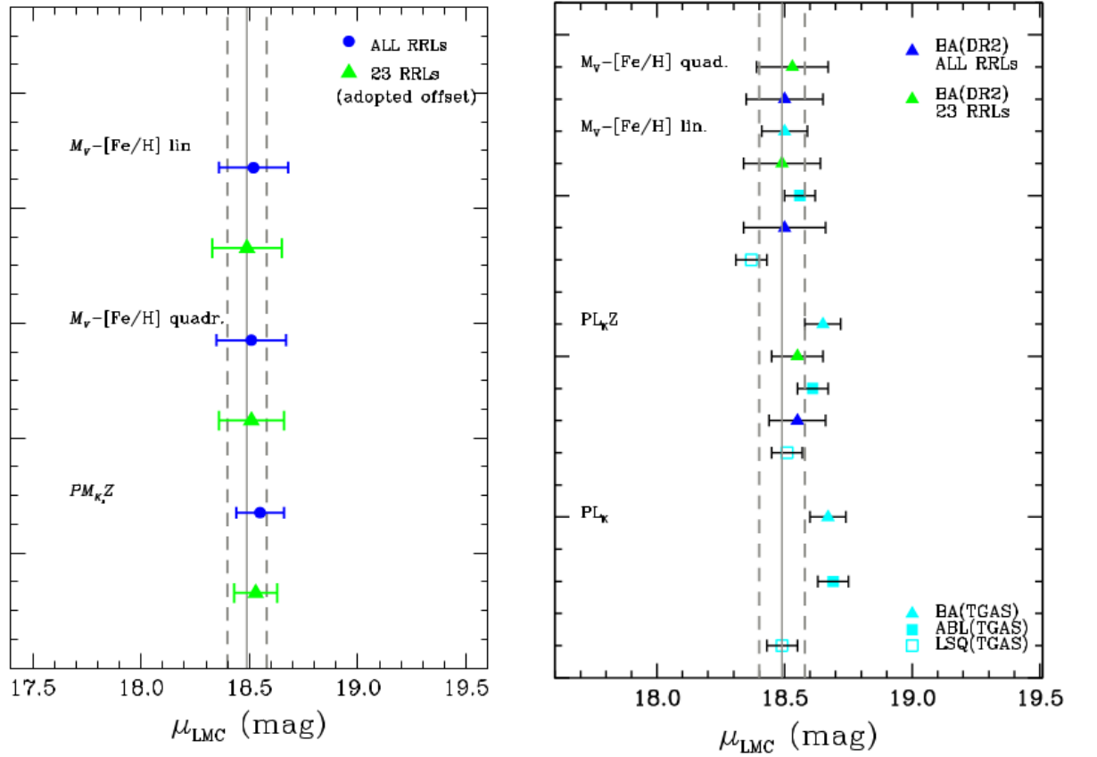
FIGURE 3.37: Left panel: LMC distance moduli obtained by fitting the DR2-based PL_{K_s}Z and M_V - [Fe/H] relations using the Bayesian approach for the whole sample of RRLs (blue filled circles) and the subset of 23 RRLs (green triangles) with an assumed constant value of the parallax offset of -0.057 mas. Right panel: As in the left panel but including LMC distance moduli derived from the TGAS-based PM_K , PM_{K_s}Z and M_V - [Fe/H] relations of RRL stars and the LSQ (cyan empty squares), ABL (cyan filled squares) and Bayesian (cyan triangles) approaches, respectively (see Sec. 3.5.6).
