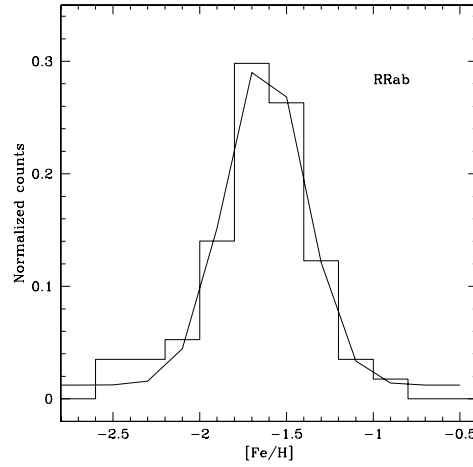
FIGURE 2.28: Metallicity distribution of And XXVII's RRab stars using the Alcock et al. (2000) method. The distribution peaks at [\text{Fe}/\text{H}] = -1.62 dex ( \sigma=0.23 dex). Figure from Cusano et al. (2017) .
