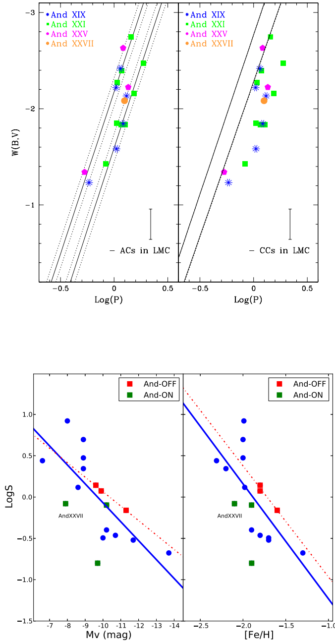
FIGURE 2.29: Upper panels: Position of V2 (orange symbol) with respect to the PW relations for ACs (left panel; Ripepi et al. 2014) and CCs in the LMC (right panel; Jacyszyn-Dobrzyniecka et al. 2016). The 95% confidence contours are shown as dotted lines. Blue, green and magenta symbols are ACs we have identified in And XIX (Cusano et al. 2013), And XXI (Cusano et al. 2015), and And XXV (Section 2.2.5). Lower panels: Specific frequency of ACs in dwarf satellites of M31 and the MW vs. absolute magnitude in the V -band (left panel) and metallicity (right panel) of the host systems. Blue filled circles are dSphs around the MW. Green and red filled square are M31 satellites respectively ON and OFF the GPoA (see Sect. 1.3 in Chapter 1 and Sect. 2.3.7 in this Chapter). Figures from Cusano et al. (2017).
