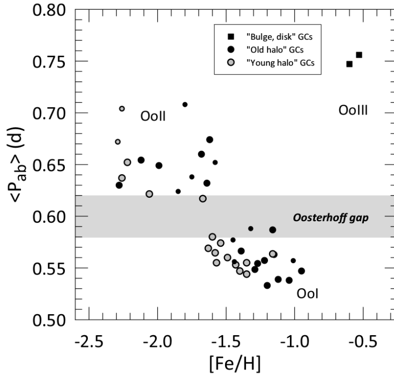
FIGURE 1.3: \langle P_{ab} \rangle of RRLs versus [Fe/H] for MW GCs. The clusters are separated into “bulge/ disk” (squares), “young halo” (filled gray circles) and “old halo” (filled black circles) subsystems, according to the Makovoz & Khan (2005) ’s classification (based on the GCs’ positions in the HB morphology-metallicity plane). Figure from Catelan (2009) .
