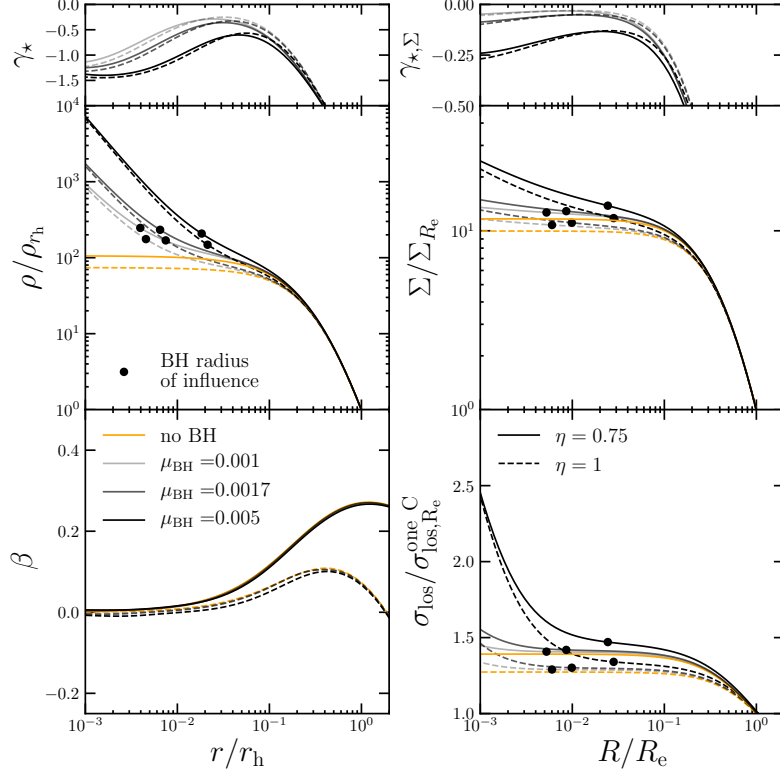
Figure 2.9: Impact of a central black hole of mass \mu_{\text{BH}} \equiv M_{\text{BH}}/M_* on one-component models. A model with \eta = 0.75 is shown by full curves while dashed curves show the radially biased model with \eta = 1 . Both models have \alpha = 0.5 . Colours indicate BH mass fraction: orange for no black hole, greys for \mu_{\text{BH}} = 0.001, 0.0017, 0.005 , respectively. Panels in the left column show from top to bottom: logarithmic slope of the stellar density profile \gamma_* ; stellar density; anisotropy parameter. Panels in the right column show: logarithmic slope of the projected density profile \gamma_{*,\Sigma} ; projected density; line-of-sight velocity dispersion. Black points mark values of R_{\text{infl}} . Densities are normalized to \rho_{r_h} \equiv \rho(r_h) , surface densities to \Sigma_{R_e} \equiv \Sigma(R_e) and line-of-sight velocity dispersions to \sigma_{\text{los},R_e}^{\text{one C}} , the line-of-sight velocity dispersion of the one component model, computed at R = R_e .
