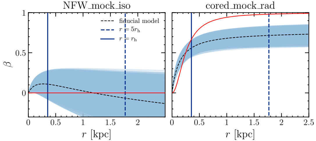
Figure D.6: Left panel: models (blue bland) and mock NFW_mock_iso (red curve) anisotropy parameter profiles. Right panel: same as the left panel, but for the mock cored_mock_rad. The full and dashed blue curves mark the position of r_h and 5r_h , respectively, where r_h is the half-mass radius of the stars (see Table D.1). The dashed black curves mark the fiducial models.
