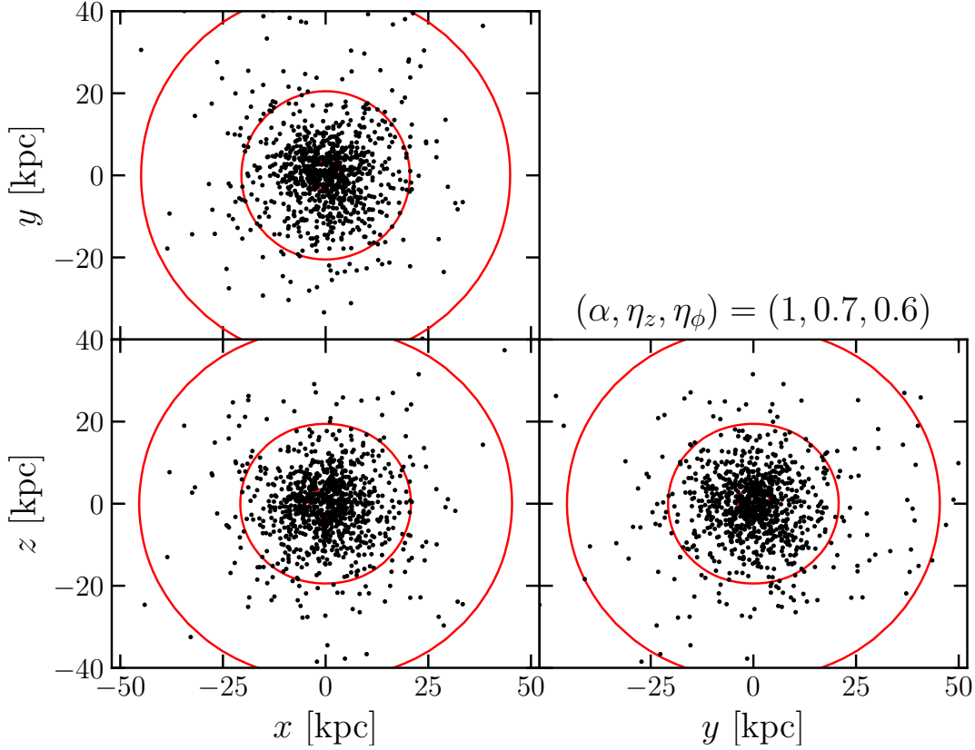
Figure 6.5: Projections on the x-y (top panel), x-z (bottom left panel) and y-z (bottom right panel) planes of the N -body realization (black points) sampled from the spherical DF with parameters (\alpha, \eta) = (1, 0.6) . In each panel we superimpose the isodensity contours of the flattened model in which the ICs are integrated (red curves). The flattened DF corresponds to the parameters (\alpha, \eta_z, \eta_\phi) = (1, 0.7, 0.6) .
