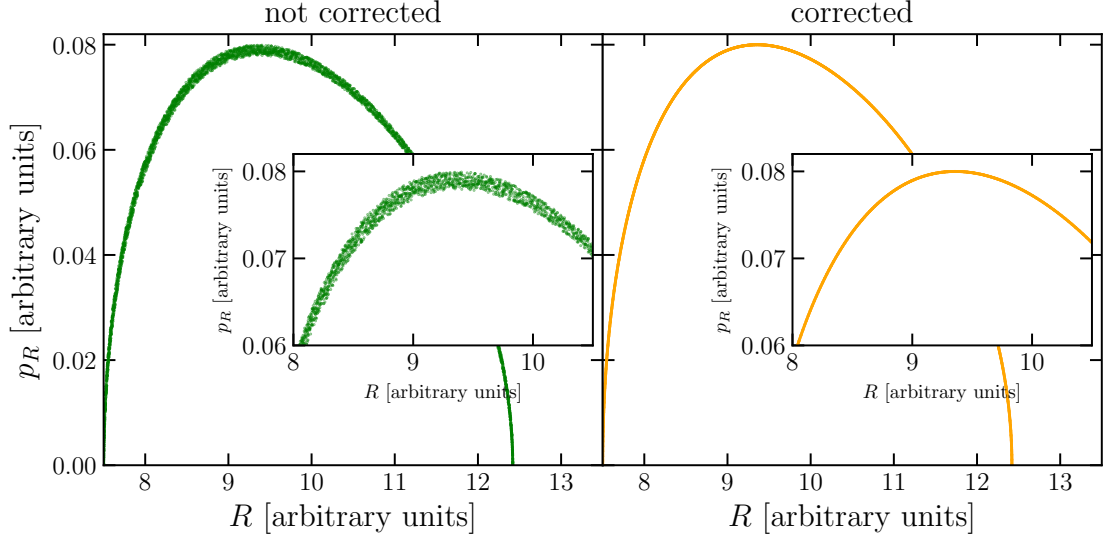
Figure 6.1: Left panel: SoS of an orbit when we do not apply the condition |z_n - z_{n+1}| < \Delta z . We plot (R, p_R) corresponding to z_{n+1} when z_n z_{n+1} < 0 . Right panel: same as the left panel, but when the condition |z_n - z_{n+1}| < \Delta z is applied. The orbit is integrated into a Miyamoto & Nagai (1975) potential, and \Delta z = 10^{-5} .
