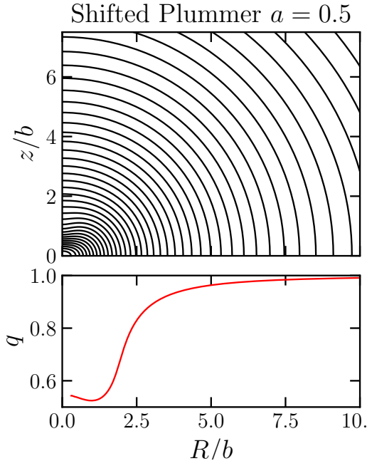
Figure 6.2: Top panel: isodensity contours in the (R, z) -plane of the shifted Plummer model (6.6), with a = 0.5 . Bottom panel: axis ratio q as a function of the semi-major axis.
