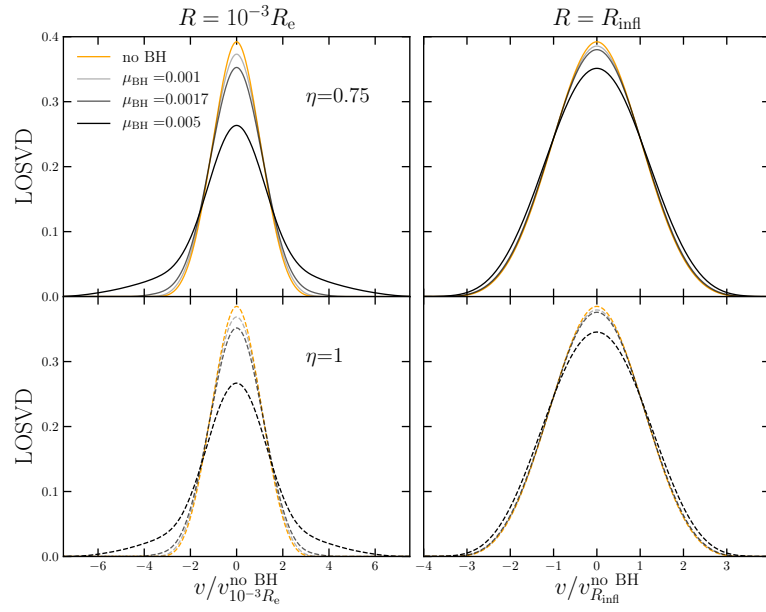
Figure 2.11: The impact of a BH on LOSVDs in one-component models: upper row an isotropic model ( \eta = 0.75 ); lower row a radially biased model ( \eta = 1 ); left column LOSVD at R = 10^{-3}R_e ; right column LOSVD at R = R_{\text{infl}} . Black hole mass fractions from zero to 0.005 are indicated by line type. Velocities are normalized to the line-of-sight velocity dispersion at the relevant radius, v_R^{\text{no BH}} , with R = 10^{-3}R_e, R_{\text{infl}} , respectively in the left and right columns. The orange curves show the LOSVD of the corresponding model with no BH. In this case R_{\text{infl}} is not defined so we plot the LOSVD at 10^{-2}R_e .
