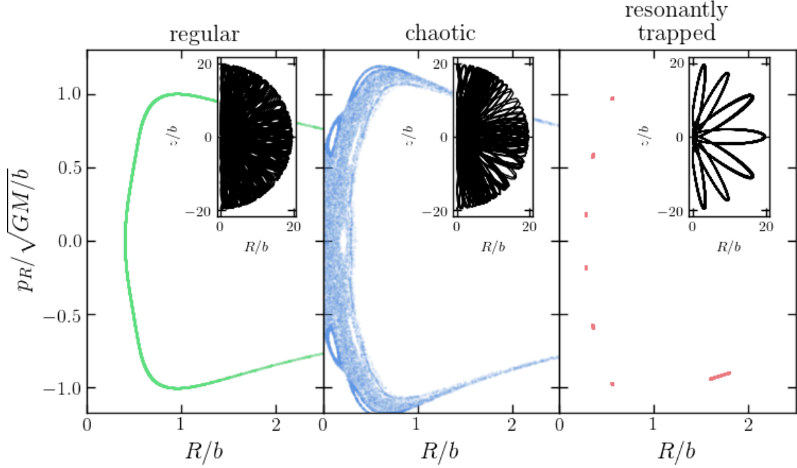
Figure 6.3: The SoS of a regular, chaotic and resonantly trapped orbits integrated in the potential (6.6), in the left, central and right panels, respectively. The small panels show the corresponding orbits in the meridional plane
