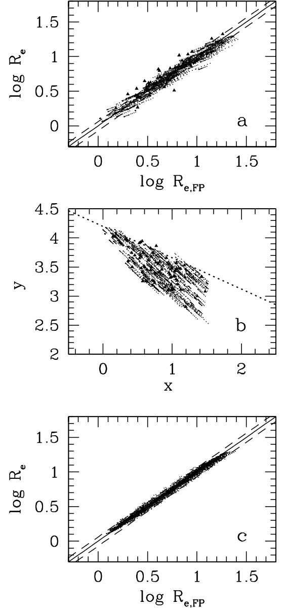
Fig. 6. Accepted models (dots) selected according to Eq. (34) and \sigma_{\text{inp}} = 0.054 , plotted in the edge-on (panel a)), and face-on (panel b)) views of the FP. For models in panel a), \sigma_{\text{int}} = 0.057 . Solid triangles are the Coma cluster galaxies in Gunn r (from JFK96). Panel c): the edge-on FP for the models selected in the “zero-thickness” approximation. Solid and dashed lines in panels a) and c) represent Eq. (1) and its intrinsic scatter, respectively. The dotted line in panel b) marks the “zone of exclusion” (JFK96).
