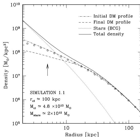
Figure 2. Final density distribution of the cluster dark, luminous and total matter in simulation 1.1. The dot-dashed curve is the initial (Hernquist) DM profile. The arrow indicates the minimum radius considered for the fit. Open symbols refer to a test simulation run to exclude numerical artefacts (see Section 2.3).
