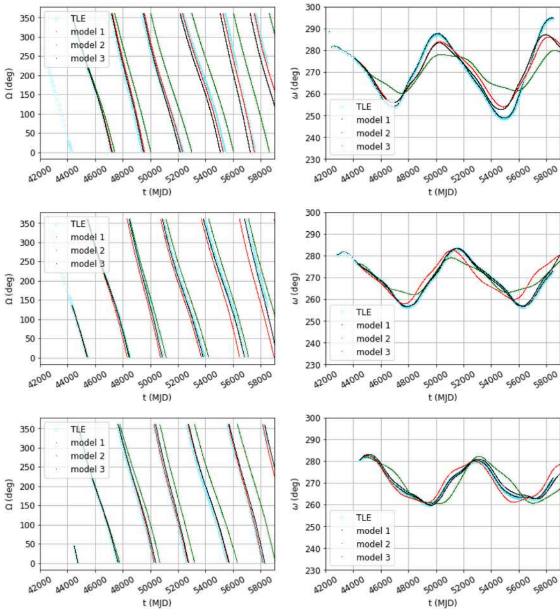
Fig. 4. Longitude of the ascending node (left) and argument of pericenter evolution (right) evolution obtained by assuming different levels of third-body perturbation of e, i, \Omega, \omega , compared against the TLE evolution for some specific examples. More details in the text. Top: #2; middle: #7; bottom: #15. The TLE evolution is displayed in cyan; the evolution obtained by applying model 1 in green; the evolution obtained by applying model 2 in red; the evolution obtained by applying model 3 in black. (For interpretation of the references to color in this figure legend, the reader is referred to the web version of this article.)
