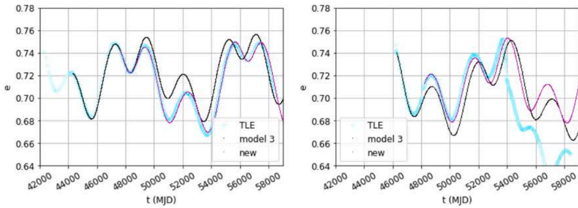
Fig. 5. On the left, in cyan the eccentricity evolution of the TLE for Molniya 2-10 (orbit #2) and the ones obtained by numerical propagation choosing two different initial conditions (black Table 1 and magenta Table 2). On the right, a similar experiment performed for Molniya 3-24 (orbit #23). (For interpretation of the references to color in this figure legend, the reader is referred to the web version of this article.)
