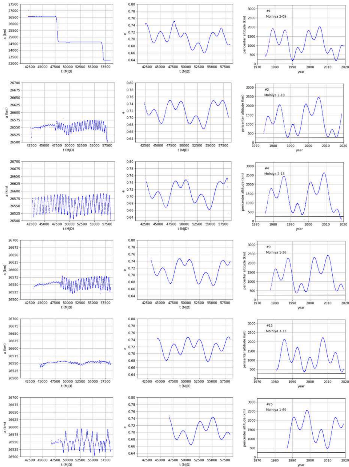
Fig. 2. Semi-major axis (left; km), eccentricity (middle) and pericenter altitude (right; km) mean evolution from the TLE data of Molniya 2-09, 2-10, 2-13, 1-36, 3-13, 1-69 (#1, 2, 4, 9, 15, 25 of Table 1). On the right, the time is displayed in decimal year for the sake of clarity; also, the black horizontal line highlights 250 km of altitude.
