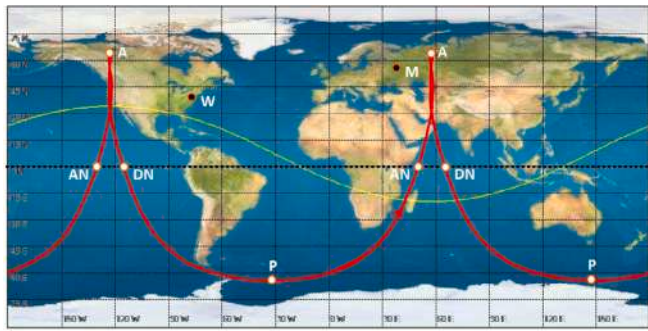
Fig. 1. An illustrative example of Molniya orbit ground track. Two 12-hr orbits are displayed to span a full day. The nominal orbital parameters are assumed, for illustrative scope, according to the template given in [12]. In particular, for our specific choice, we set the relevant geometric orientation parameters (i, \omega) = (63.4, 270) deg, with orbit scale length parameters (in km) (a, h_p, h_a)_{km} = (26560, 1000, 39360) . This implies an eccentricity e = 0.72 and a period P = 720 min. Note the extremely asymmetric location of the ascending (“AN”) and descending (“DN”) nodes, due to the high eccentricity of the orbit, and the perigee (“P”), always placed in the Southern hemisphere. Along the two daily apogees (“A”), the satellite hovers first Russia and then Canada/US. The visibility horizon (aka the “footprint”) attained by the Molniya at its apogee over Russia, is above the displayed yellow line. (For interpretation of the references to color in this figure legend, the reader is referred to the web version of this article.)
