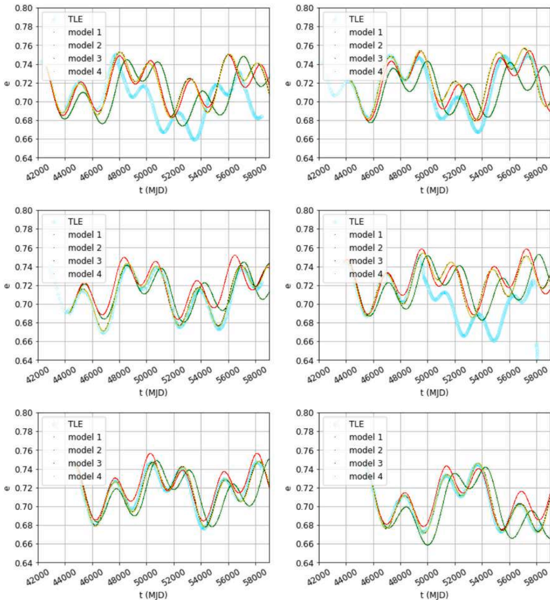
Fig. 3. Eccentricity evolution obtained by assuming different levels of third-body perturbation of e, i, \Omega, \omega , compared against the TLE evolution for some specific examples. More details in the text. Top: orbits #1 and #2; middle: #7 and #13; bottom: #15 and #19. All the other orbits are shown in the “SUPPLEMENTARY MATERIAL 2”. The TLE evolution is displayed in cyan; the evolution obtained by applying model 1 in green; the evolution obtained by applying model 2 in red; the evolution obtained by applying model 3 in black; the evolution obtained by applying model 4 in yellow. (For interpretation of the references to color in this figure legend, the reader is referred to the web version of this article.)
