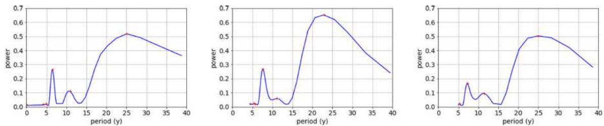
Fig. 7. Example of the results obtained by applying a Lomb–Scargle procedure to the eccentricity series. From left to right: Molniya 2-09, 2-10, 2-29 (orbit #1, 2, 3, respectively). In red, the dominant terms. (For interpretation of the references to color in this figure legend, the reader is referred to the web version of this article.)
