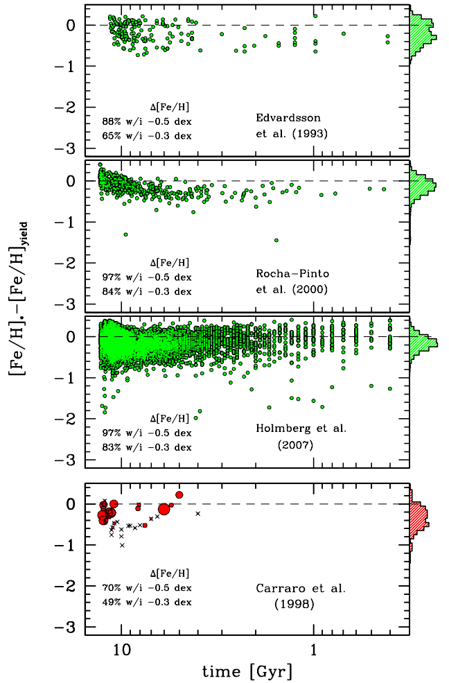
Figure 8. The observed metallicity distribution of stars in the solar neighbourhood. The displayed quantity is \Delta[Fe/H] = [Fe/H]_* - [Fe/H]_{\text{yield}} \equiv \log(Z_{\text{gas}}/Z) . Different stellar samples have been considered from the work of Edvardsson et al. (1993), Rocha-Pinto et al. (2000), and Holmberg, Nordström, & Andersen (2007), from top to bottom, as labelled in each panel. The lower panel displays the same trend for a sample of open stellar clusters, after Carraro, Ng, & Portinari (1998). The different Galactocentric distance for these systems is indicatively marked by the dot size (i.e. the smallest the dot, the largest the distance from the Galaxy center). For each distribution, the relative fraction of stars within a -0.3 and -0.5 dex \Delta[Fe/H] residual is reported in each panel. A cumulative histogram of the data is also displayed, along the right axis, in arbitrary linear units.
