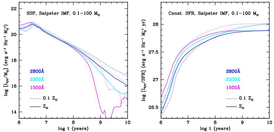
Figure 2: ( Left panel ) Time dependence of the UV luminosity of an SSP with initial mass 1 M_{\odot} , formed with a Salpeter IMF in the range 0.1 - 100 M_{\odot} , measured at three wavelengths, 1,500 \text{ \AA} , 2,300 \text{ \AA} , and 2,800 \text{ \AA} , and computed with the stellar population synthesis models of Conroy et al. (2009): ( solid lines ) solar metallicity ( Z_* = 0.02 ), ( dashed lines ) 1/10 th solar metallicity ( Z_* = 0.002 ). ( Right panel ) Time dependence of the UV luminosity per unit SFR for a model with a constant SFR, shown for the same UV wavelengths and metallicities as in the left panel.
