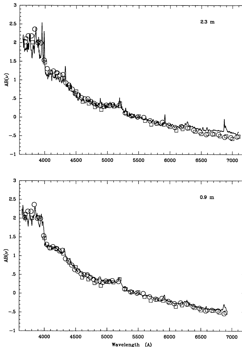
FIG. 1.—Comparison of mean spectra of giant elliptical galaxies observed here ( solid lines ) with spectrophotometric scanner observations by Schild & Oke (1971; open squares ) and Whitford (1971; open circles ). See text for definition of the normalized flux AB(\nu) .
