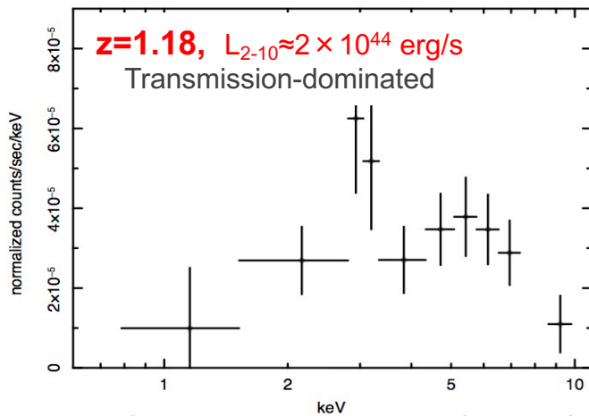
Observed flat X-ray spectra → reflection/transmission dominated, strong iron K \alpha line
