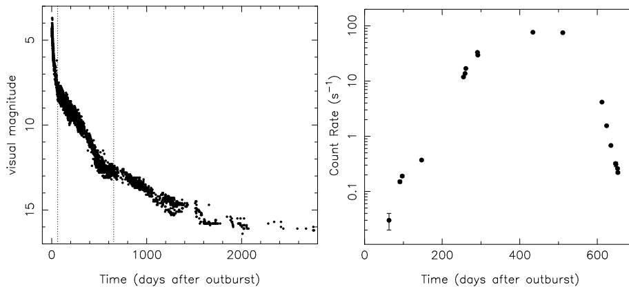
Fig. 10.8. Optical light curve ( left ) based on VSOLJ, VSNET and AFOEV visual estimates and X-ray light curve ( right ; from Krautter et al. 1996) based on ROSAT /PSPC data (0.1–2.4 keV) of the CN V1974 Cyg (Nova Cyg 1992). The start of the outburst is at Feb 19, 1992. In the left panel we indicate with dotted lines the timespan of the right panel.
