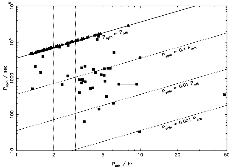
Fig. 10.5. The P_{\text{spin}} versus P_{\text{orb}} diagram of magnetic CVs. Polars are indicated by triangles; IPs are indicated by squares.
