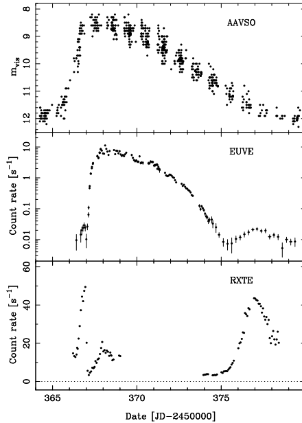
Fig. 10.1. Simultaneous AAVSO, EUVE and RXTE observations of SS Cyg throughout outburst. Note that the RXTE light curve is plotted on a linear scale in order to emphasize the timing of the sharp transitions. From Wheatley et al. (2003).
